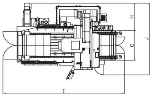
Technical drawing of the front view of a machine tool. The drawing shows a complex assembly with various components, including a large cylindrical body, a central vertical structure, and a base. Dimensions are indicated by lines and labels: 'I' for the total width, 'J' for the total height, 'G' for the height of the central section, and 'H' for the height of the base section.
