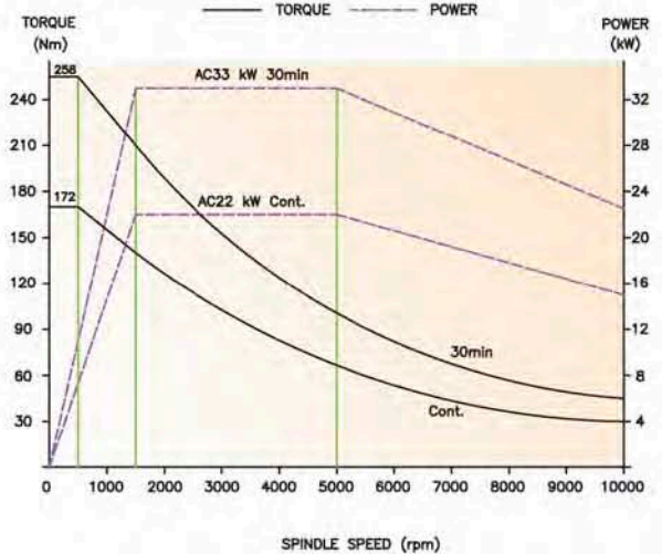
CAT-50 Gear Head 10,000 rpm (Siemens)
